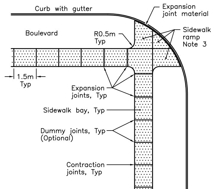
JOINT LAYOUT
