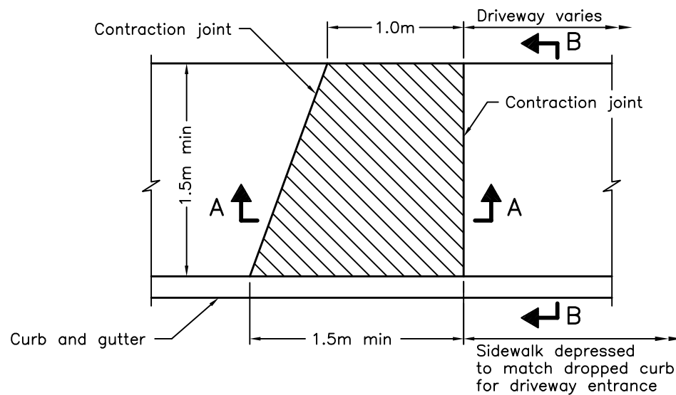
FULLY DEPRESSED
