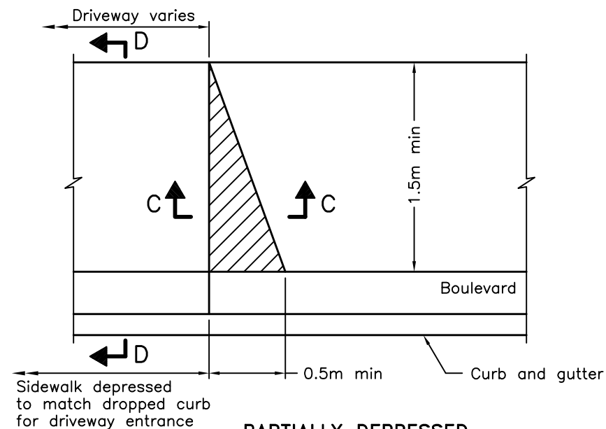
PARTIALLY DEPRESSED
